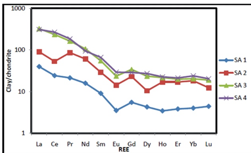
Fig. 6: Chondrite normalized plot of Rare Earth Elements of Isan clay
