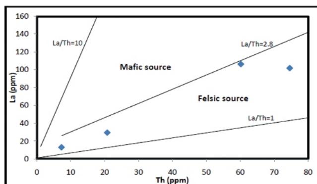
Fig. 5: La versus Th plot for Isan clay (after Nyakairu and Koeberl, 2001)
