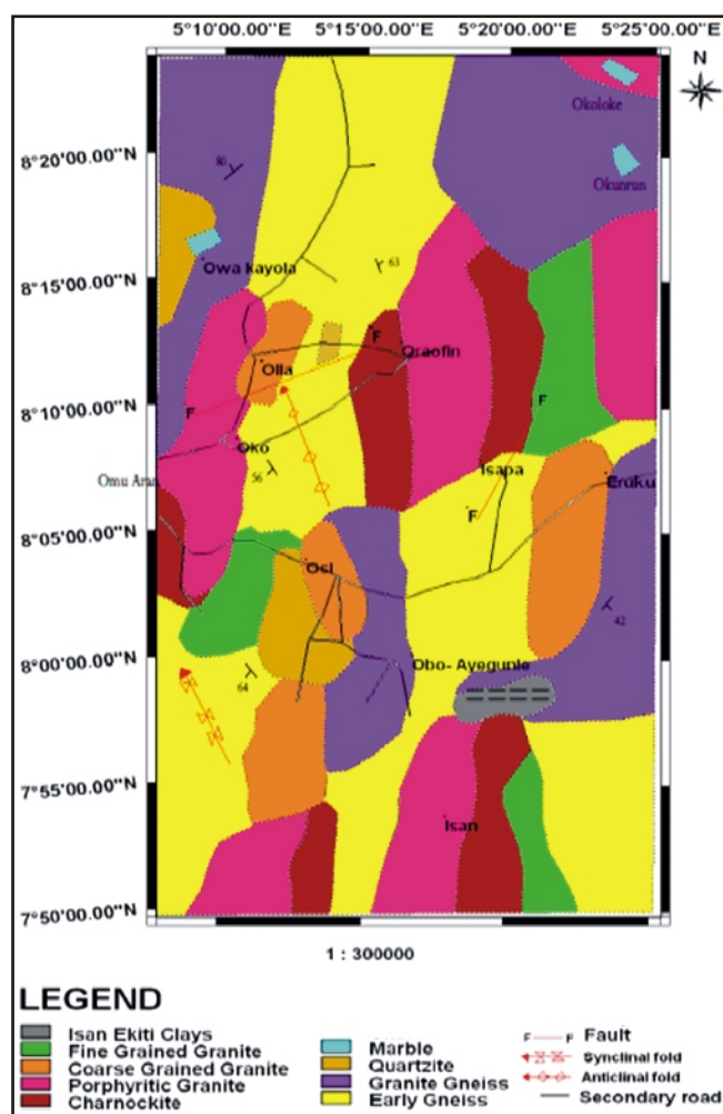
Fig. 2: Geological map of Isan area (Odewumi, 2016)
