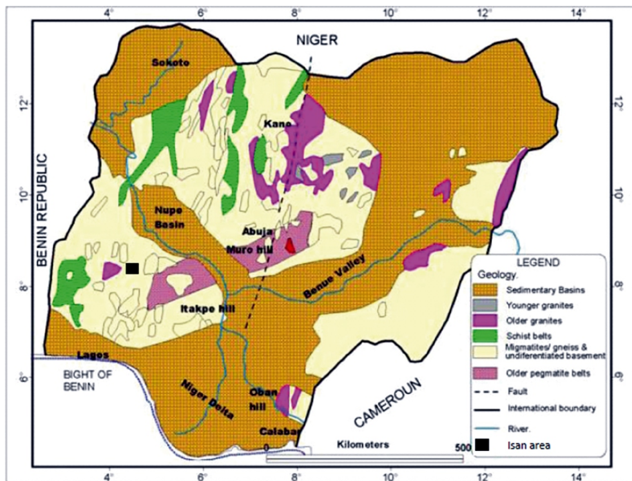
Fig. 1: Geological map of Nigeria showing location of the Isan area (Geological Survey of Nigeria, 2005)
