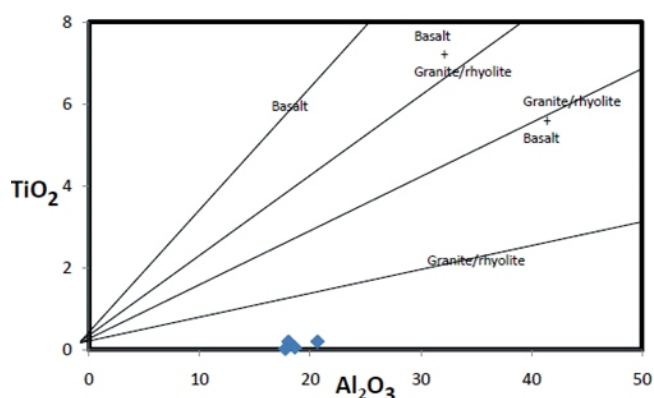
Fig. 4: TiO_2 (wt%) versus Al_2O_3 (wt%) binary plot of Isan clay (after Ekosse, 2001)
