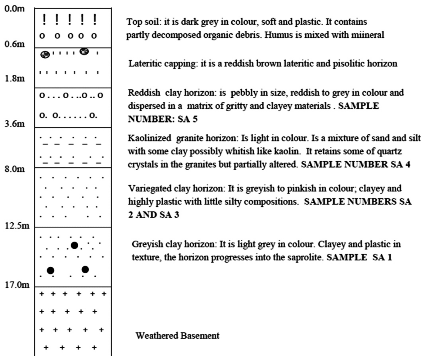
Fig. 3: Profile Section of Isan Clay
